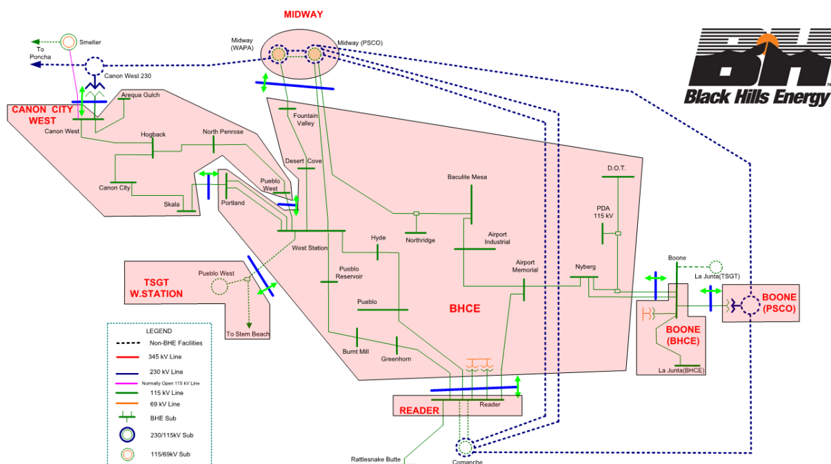
Figure 7-2 Existing Black Hills Transfer Path Map
