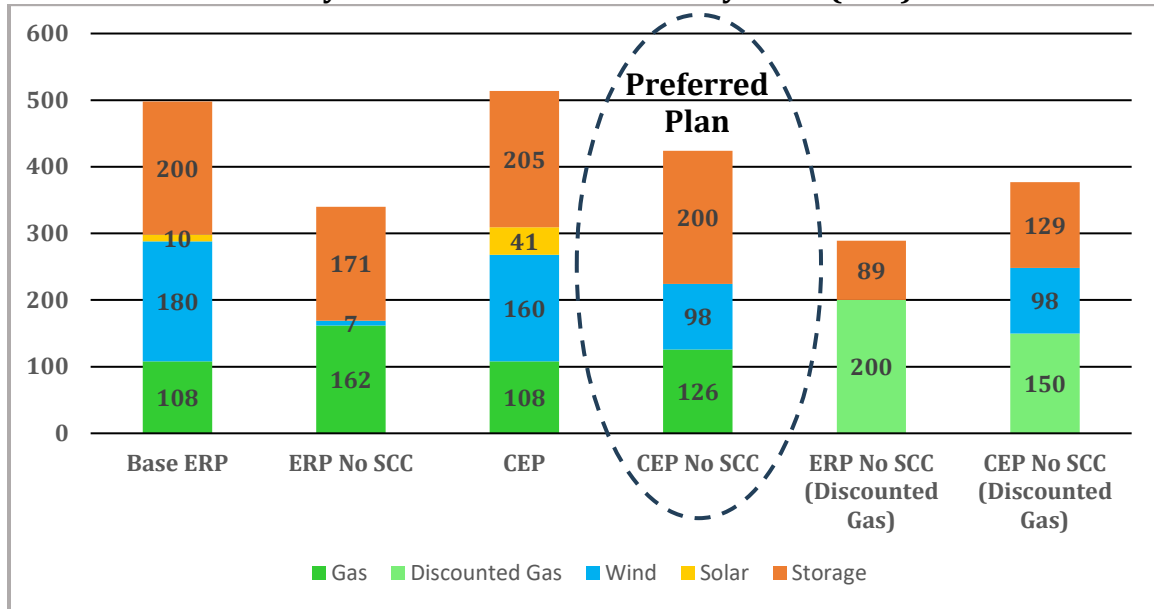
Figure 8-3 Optimal Expansion Plans – Core and Gas Alternative CEP and ERP Scenario Analysis – Resource Additions by 2032 (MW)
