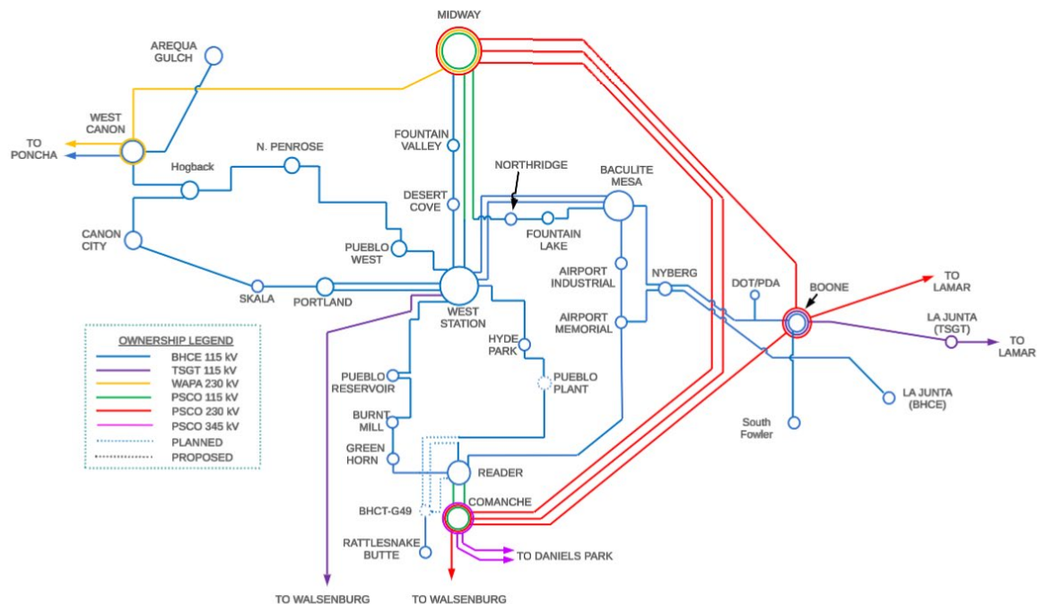
Figure 7-1 Existing Black Hills Transmission System
