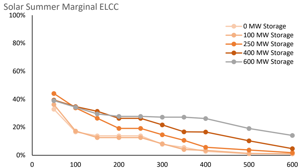
Figure 6-2 Calculated Summer Solar ELCC 39
