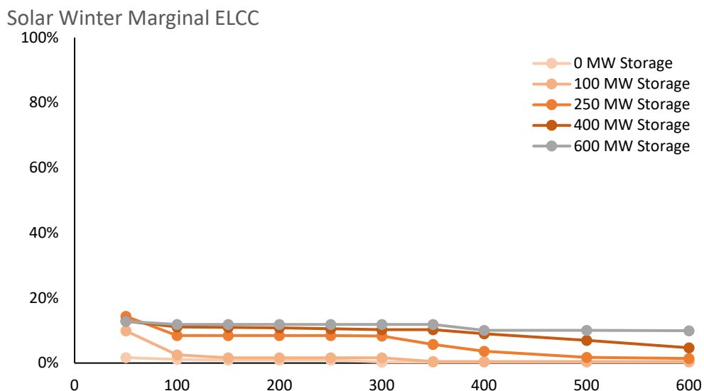
Figure 6-3 Calculated Winter Solar ELCC 40
