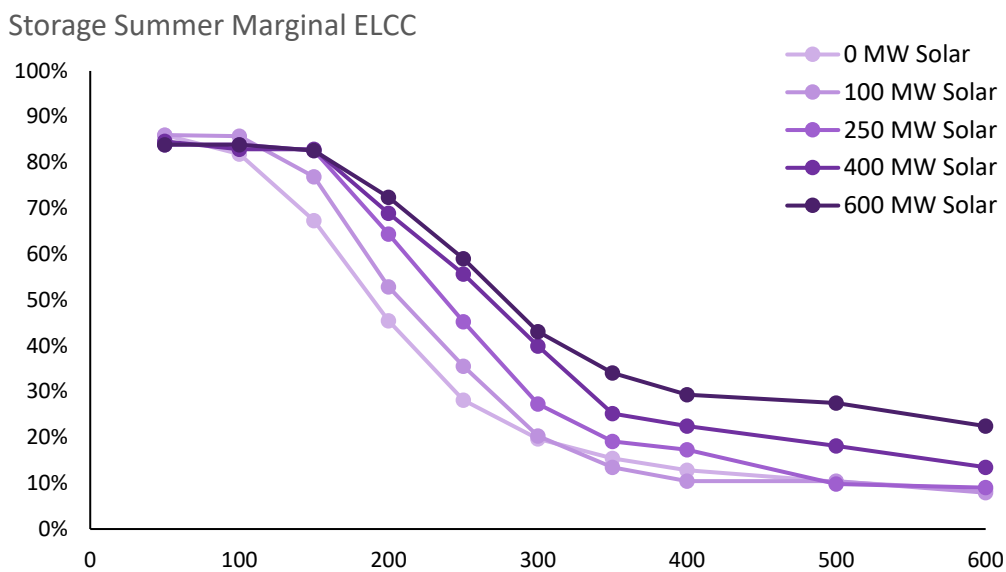
Figure 6-4 Calculated Summer Storage ELCC 41
