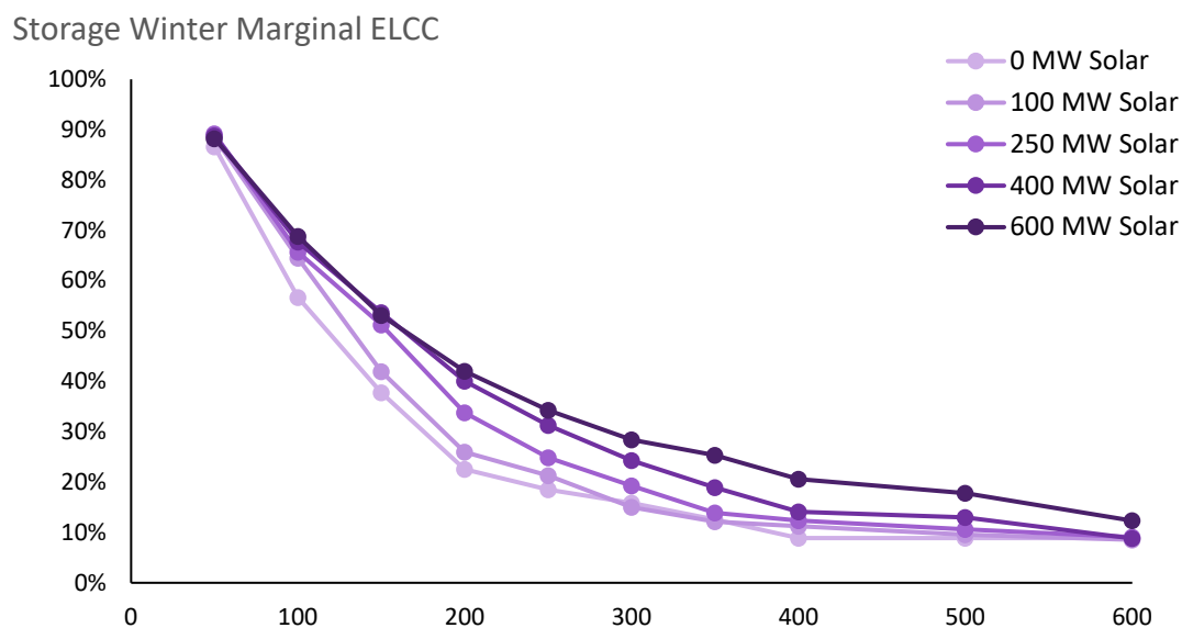
Figure 6-5 Calculated Winter Storage ELCC 42
