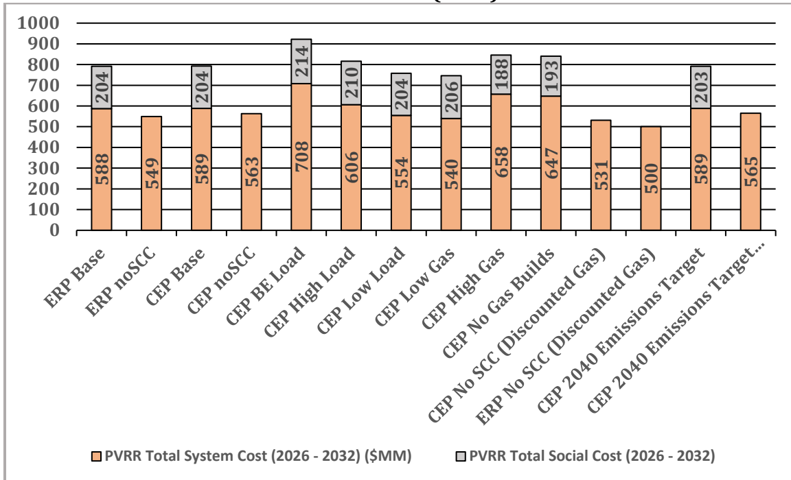
Figure 8-1 Base ERP and Scenarios – Deterministic RAP PVRRs (2026-2032) 7 Year PVRR ($MM)
