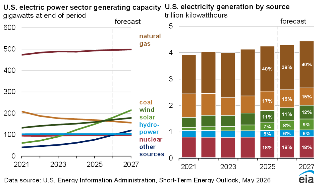
Figure 2-2 EIA's Historic and Projected Electric Generation by Fuel Source
