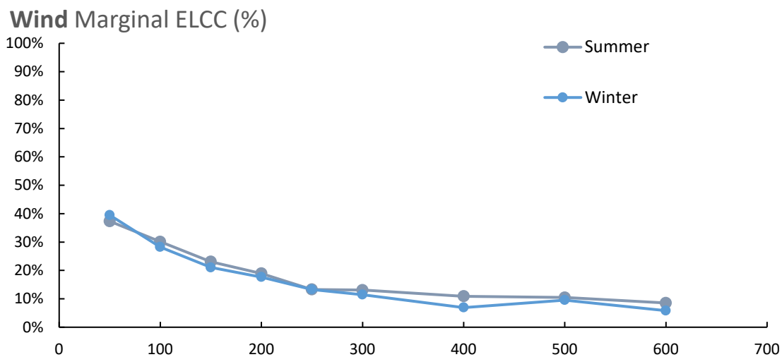
Figure 6-6 Calculated Summer and Winter Wind ELCC 43
