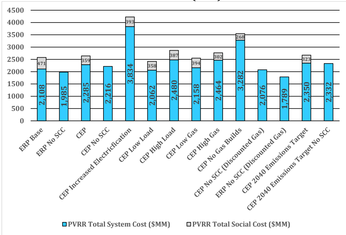
Figure 8-2 Base ERP and Scenarios – Deterministic PVRs (2026-2050) 25 Year PVR ($MM)
